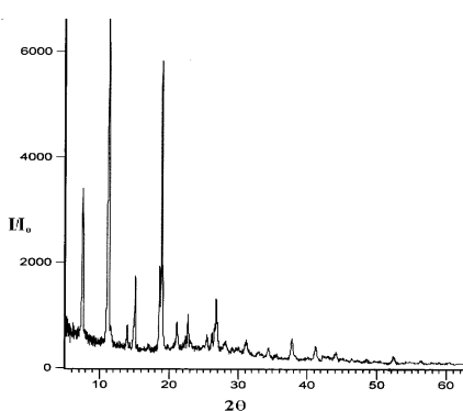
Fig. 5. X-ray spectrum of \text{PdL}.\text{H}_2\text{O}.\text{Cl}
